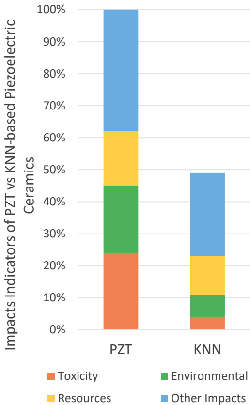
Total impact indicators of PZT and KNN-based piezoceramics. 4
