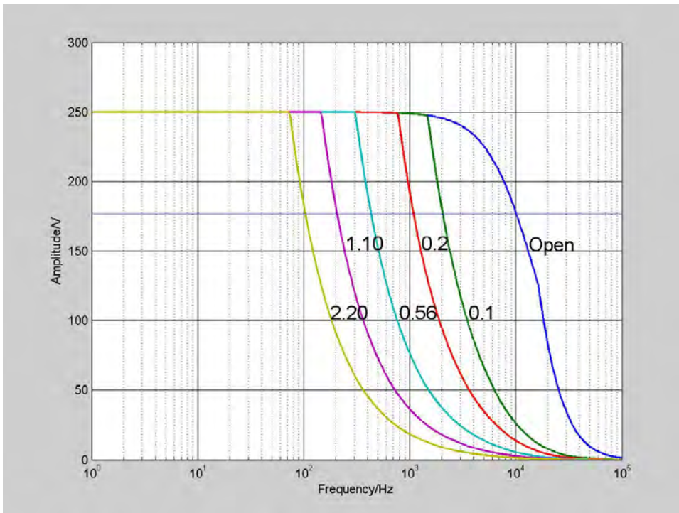
E-536.3x: Operating limits with various piezo loads, capacitance values in μF
