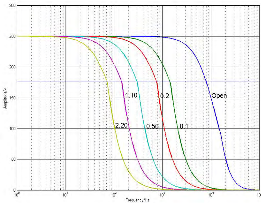
E-536.3xH: Operating limits with various piezo loads, capacitance values in μF
