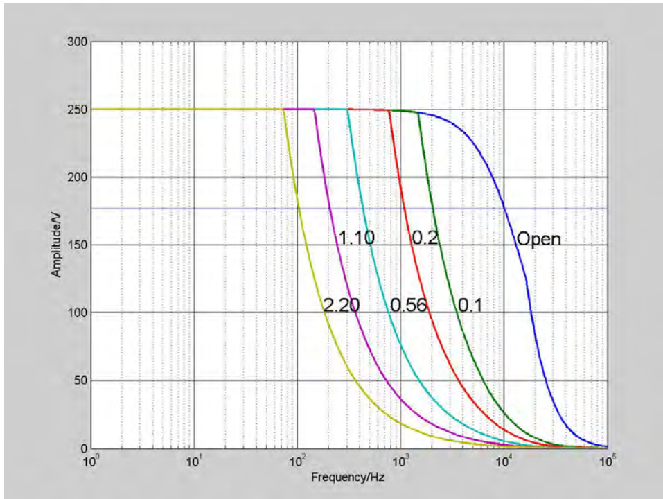
E-536.3x: Operating limits with various piezo loads, capacitance values in \mu F
