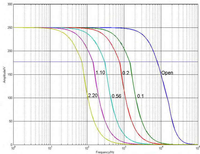
E-536.3xH: Operating limits with various piezo loads, capacitance values in \mu F
