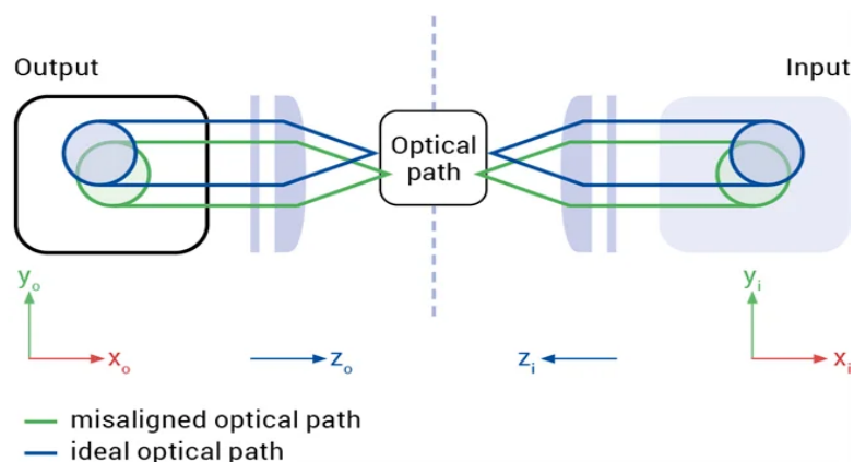
Figure 1. Testing and packaging today's photonic devices can be challenging across multiple DOF. The alignment of multi-channel devices, such as fiber-optical arrays, used to be a slow, repetitive process before modern parallel algorithms were developed. Image Credit: PI (Physik Instrumente) LP
