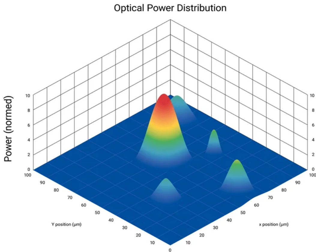
Figure 2. Power distribution of an optical component shows multiple peaks. Modern algorithms and precision mechanics can help determine the main mode and find the exact peak quickly. Image Credit: PI (Physik Instrumente) LP
