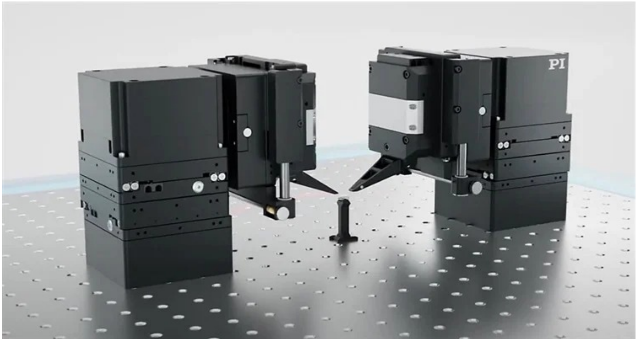
Figure 9. The F-141, dual-sided, PILightning-enabled fiber alignment system - dubbed PINovAlign - is designed to provide highest performance with the most compact footprint. It is available in 3-, 4-, and 6-axis configurations and provides exceptional throughput advantages in fiber-array applications. Image Credit: PI (Physik Instrumente) LP
